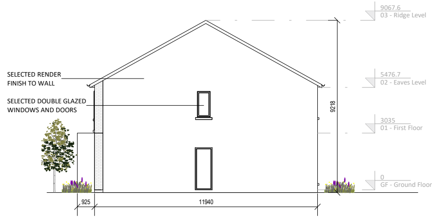
② H05 Side Elevation 1 : 200
