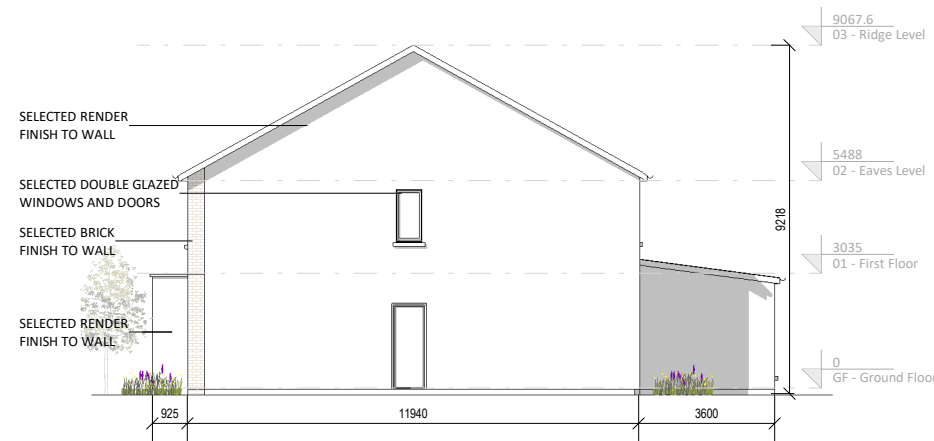
⑥ H05 Side Elevation (Extended) 1 : 200
