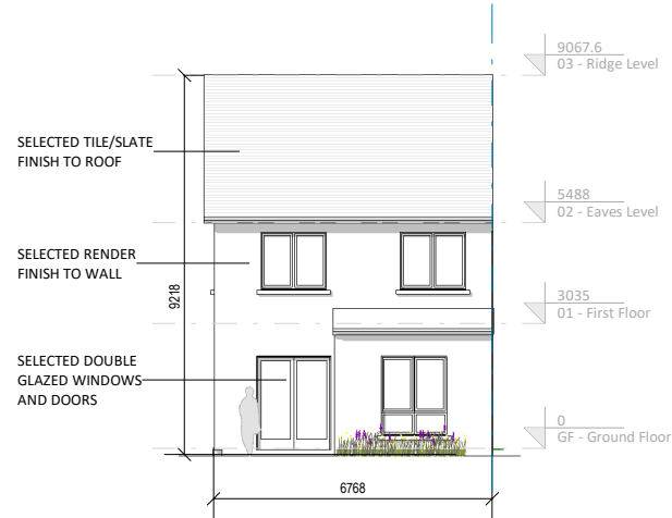
④ H05 Rear Elevation (Extended) 1 : 200
